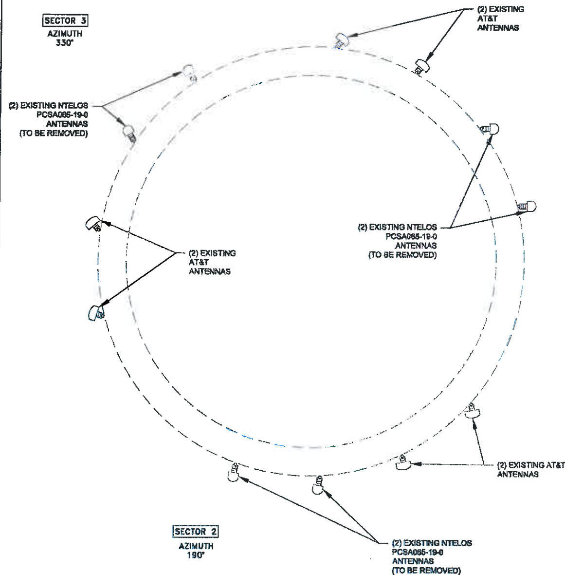
EXISTING ANTENNA CONFIGURATION NOT TO SCALE
