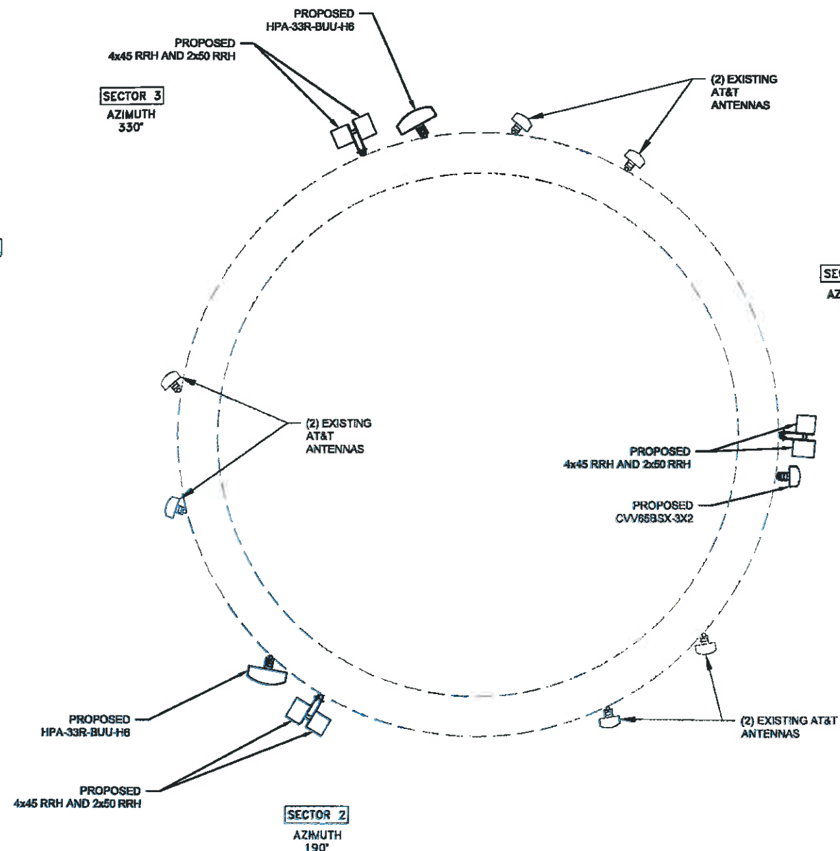
PROPOSED ANTENNA CONFIGURATION NOT TO SCALE
