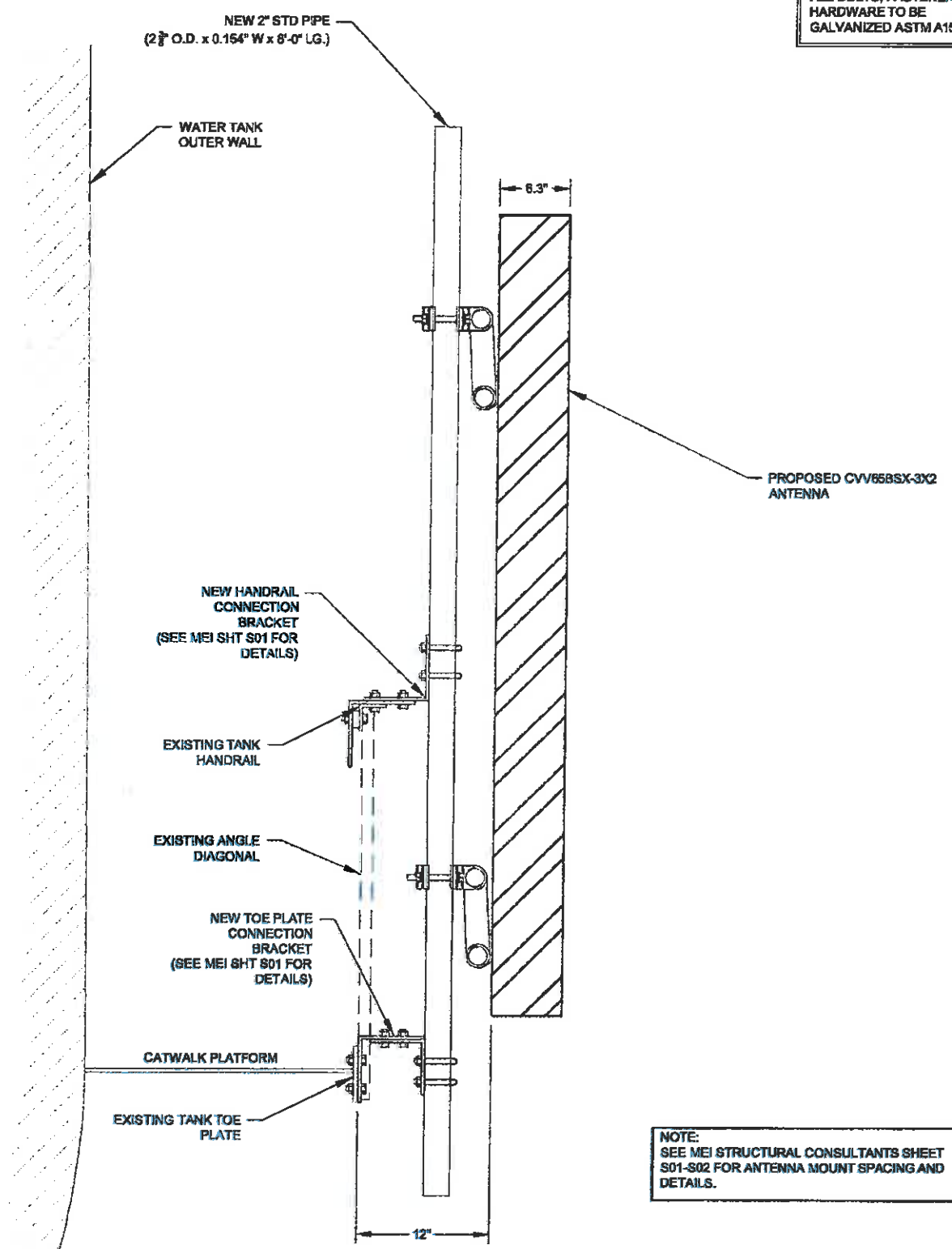
PROPOSED ANTENNA MOUNTING DETAIL (ELEVATION VIEW) NOT TO SCALE
